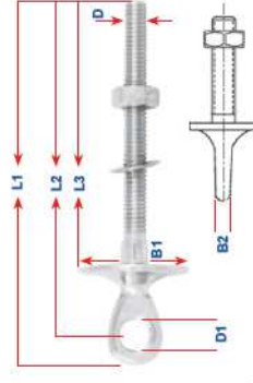
Art. n° 8032 Golfare stampato lucido Eye bolt, polished
